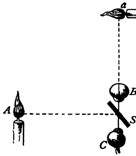
FIG. 71.—Principle of the ophthalmoscope. (Fick.)
